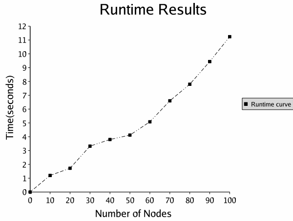
Fig. 5. Runtime Performance
